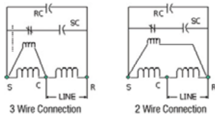
Figure 1. Wiring Configurations
